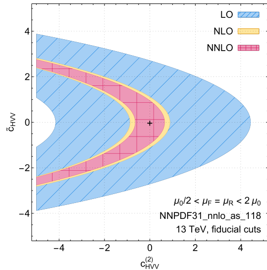
Figure 2. Same as Fig. 1 but for combinations involving the CP-odd anomalous coupling \tilde{c}_{HVV} . See text for details.
