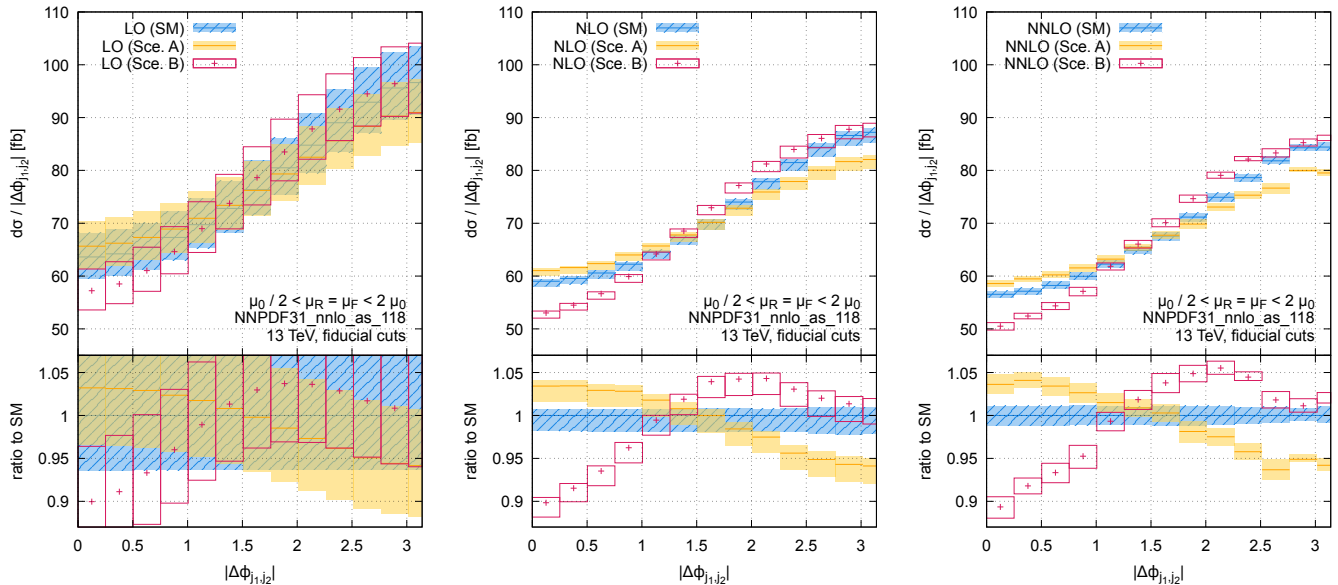
Figure 6. Same as Fig. 4 but for the absolute value of the azimuthal angle difference between the forward and backward VBF tag jets. See text for details.
