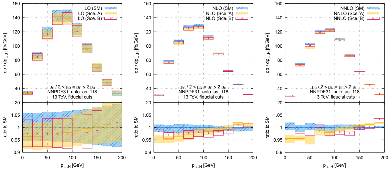
Figure 3. Transverse momentum distributions of the Higgs boson for LO (left), NLO (middle) and NNLO (right) QCD predictions. For each plot, the upper pane displays the SM (hashed blue), scenario A (solid yellow) and scenario B (red boxes) results as defined in the main text. The lower pane shows the ratio of these results to the SM result at central scale. The lines indicate the central renormalization and factorization scale choice, and the bands indicate the envelope of the results at different scales. See text for details.
