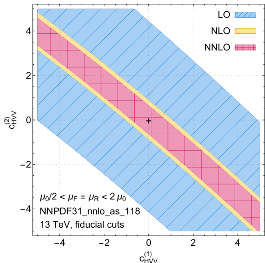
Figure 1. Allowed combinations of anomalous couplings c_{HVV}^{(1)} and c_{HVV}^{(2)} where the residual scale uncertainty band overlaps with SM prediction at the 13 TeV LHC. The color coding describes LO (hashed blue), NLO (yellow) and NNLO (squared red) calculations. The SM result is shown as black cross. See text for details.
