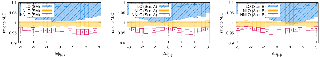
Figure 5. LO (hashed blue) and NNLO (red boxes) predictions for the azimuthal separation between the forward and backward VBF tag jets, divided by the corresponding NLO (solid yellow) result. Left pane: Standard Model. Middle pane: Scenario A. Right pane: Scenario B. The envelope represents scale variation uncertainties. See text for details.
