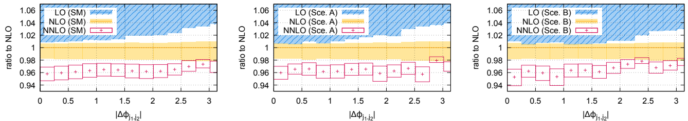
Figure 7. Same as Fig. 5 but for the absolute azimuthal angle separation between the forward and backward VBF tag jets. See text for details.
