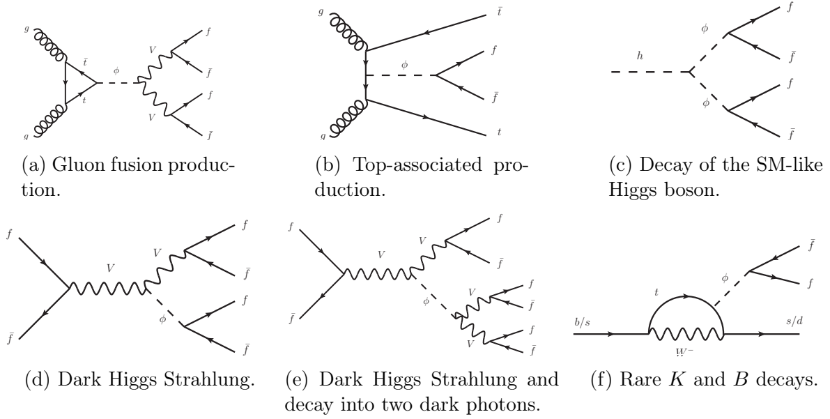
Figure 3.1: Feynman diagrams depicting the leading Dark Higgs search channels. Depending on context, f denotes either a SM fermion or a DM particle, and V denotes either a SM gauge boson or a dark photon.
