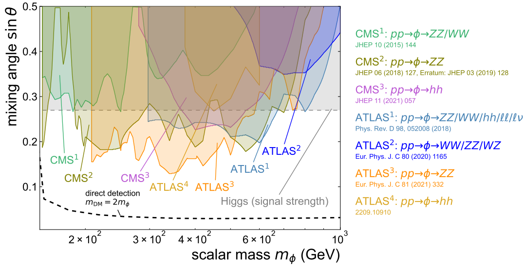
Figure 5.1: 95 % CL upper limits on the mixing angle \sin \theta as function of scalar mass m_S for heavy dark Higgs bosons from CMS [56, 57, 61] and ATLAS [58, 59, 60, 62]. For limits from Higgs signal strength see Sec. 4. For limits from direct detection experiments see Sec. 10.2. Constraints colored in gray with dashed outline are reinterpretations not performed by the experimental collaborations and without access to raw data.
