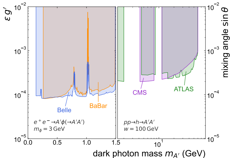
Figure 6.1: Constraints on dark Higgs models arising from searches for dark photons. The upper limits from Belle (90 % CL [115]) and BaBar (90 % CL [116]) in the left half of the plot result from searches for e^+e^- \rightarrow A'\phi(\rightarrow A'A') , which constrains the product of the kinetic mixing parameter \epsilon and the dark gauge coupling g' . The upper limits from CMS (95 % CL [117]) and ATLAS (95 % CL [118]) in the right half of the plot result from searches for pp \rightarrow h \rightarrow A'A' , which constrains the Higgs mixing parameter \sin \theta .
