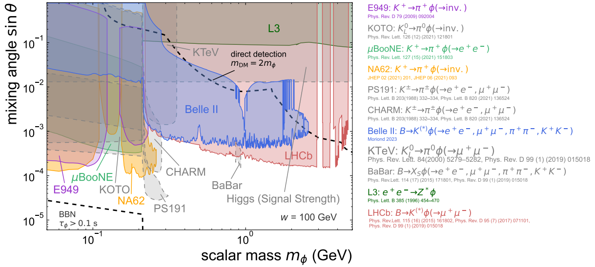
Figure 5.3: Upper limits on the mixing angle \sin \theta as function of scalar mass m_S from PS191 (90 % CL [79]), E949 (90 % CL [76]), NA62 (90 % CL [74, 75]), MicroBooNE (95 % CL [80] and this work), KOTO (90 % CL [86] and this work), KTeV (90 % CL [83]), L3 (95 % CL [64] and this work), CHARM (95 % CL [81, 24]), LHCb (95 % CL [71, 72, 24]), Belle II (95 % CL [68]), BaBar (90 % CL [69, 24]). For limits from Higgs signal strength see Sec. 4. For limits from BBN see Sec. 10.1. For limits from direct detection experiments see Sec. 10.2. Constraints colored in gray with dashed outline are reinterpretations not performed by the experimental collaborations and without access to raw data.
