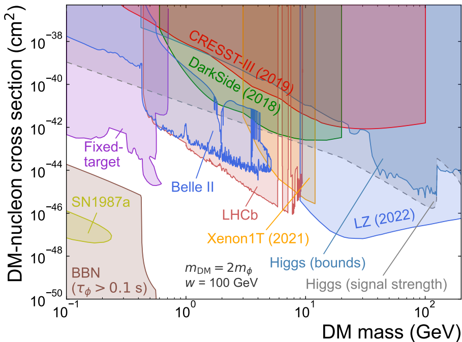
Figure 10.2: Upper limits on the spin-independent DM-nucleon cross section \sigma as function of DM mass m_{\text{DM}} for light dark Higgs bosons from CRESST-III [190], DarkSide [191], XENON1T [192], and LZ [189]. For limits from direct dark Higgs searches, limits from flavour experiments and fixed-target experiments see Sec. 5, and for limits from Higgs signal strength see Sec. 4. We also indicate the approximate lower bound on \sin\theta imposed by BBN [160] and the parameter region excluded by the duration of the neutrino signal from SN1987a [193]. Constraints colored in gray with dashed outline are reinterpretations not performed by the experimental collaborations and without access to raw data.
