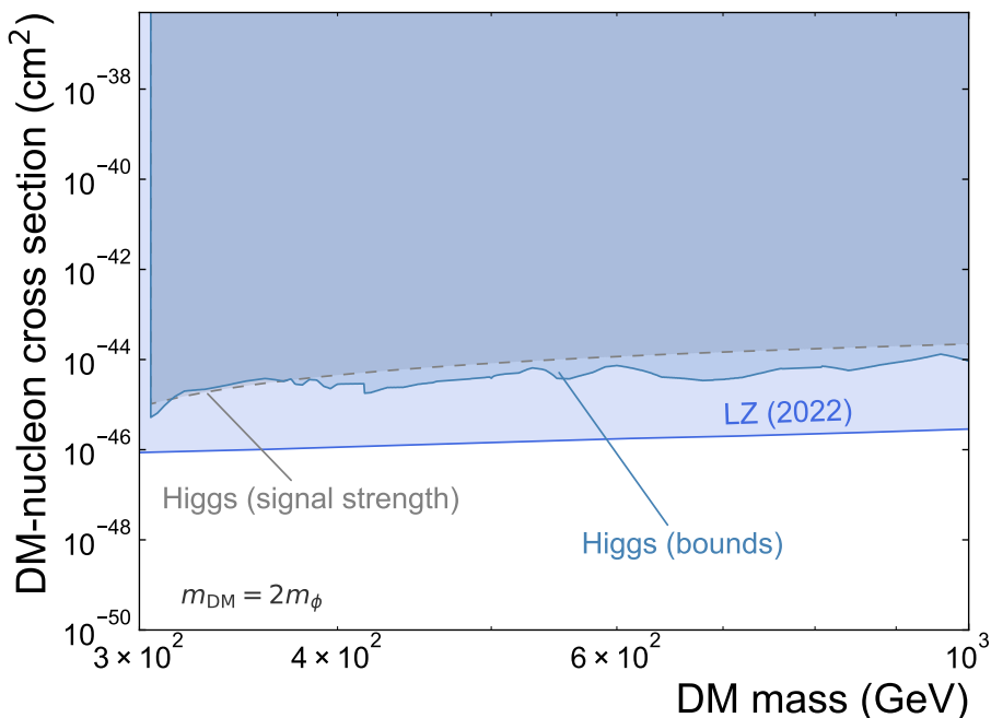
Figure 10.1: Upper limits on the spin-independent DM-nucleon cross section \sigma as function of DM mass m_{\text{DM}} for heavy dark Higgs bosons from LZ [189]. For limits from direct dark Higgs searches see Sec. 5, and for limits from Higgs signal strength see Sec. 4. Constraints colored in gray with dashed outline are reinterpretations not performed by the experimental collaborations and without access to raw data.
