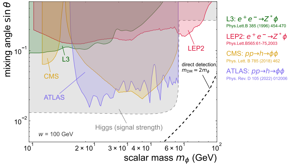
Figure 5.2: 95% CL upper limits on the mixing angle \sin\theta as function of scalar mass m_S for light dark Higgs bosons from CMS [66], ATLAS [67], LEP2 [65], and L3 [64]. For limits from Higgs signal strength see Sec. 4. For limits from direct detection experiments see Sec. 10.2. Constraints colored in gray with dashed outline are reinterpretations not performed by the experimental collaborations and without access to raw data.
