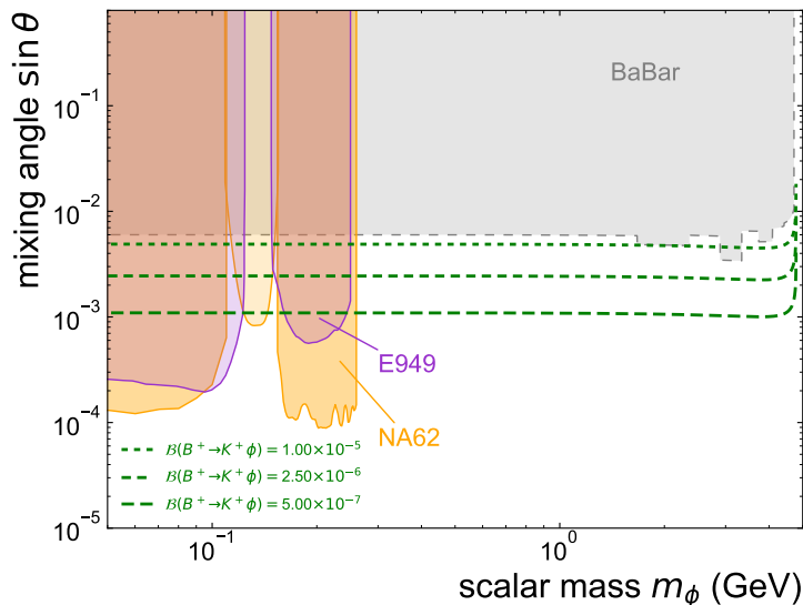
Figure 7.1: Upper limits on the mixing angle \theta as function of scalar mass m_\phi from NA62 (95 % CL [79]), E949 (90 % CL [76]), and BaBar (95 % CL [122] and this work). Constraints colored in gray with dashed outline are reinterpretations not performed by the experimental collaborations and without access to raw data. The green dashed lines indicates the parameter combinations that correspond to branching ratios between 5 \times 10^{-7} \leq \mathcal{B}(B^+ \rightarrow K^+ \phi) \leq 1 \times 10^{-5} .
