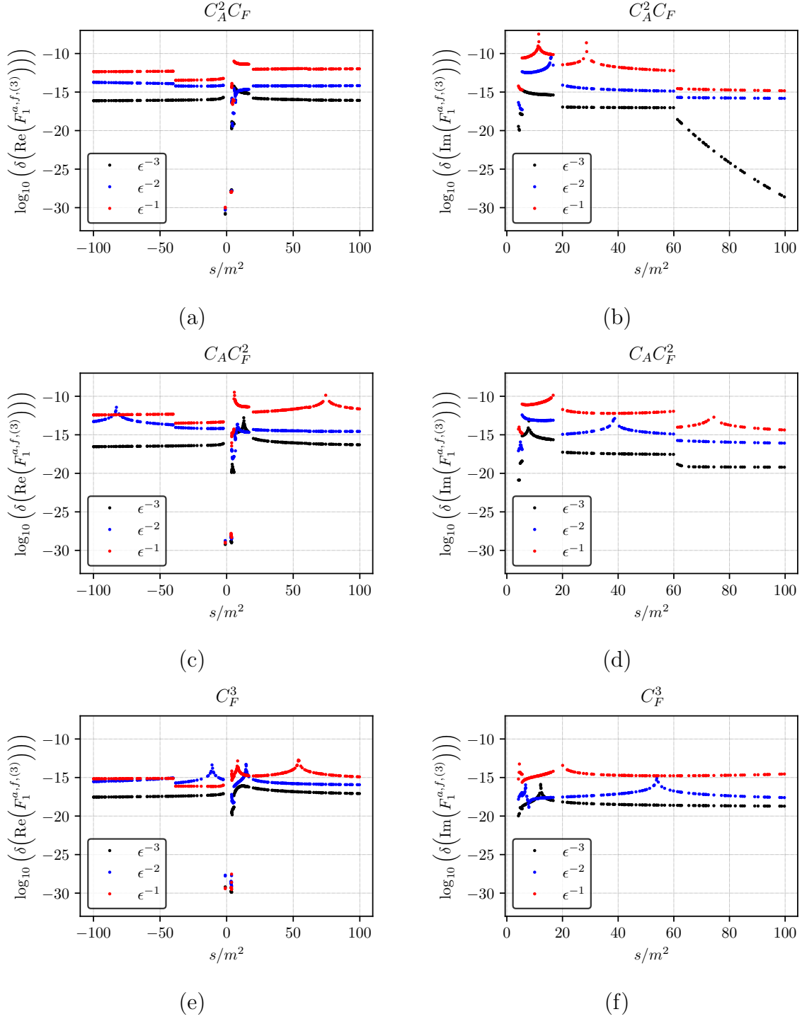
Figure 12: Relative cancellation of the real, (a), (c), (e), and imaginary parts, (b), (d), (f), of the poles for the non-fermionic colour structures of F_1^{a,f,(3)} , c.f. Eq. (31).
