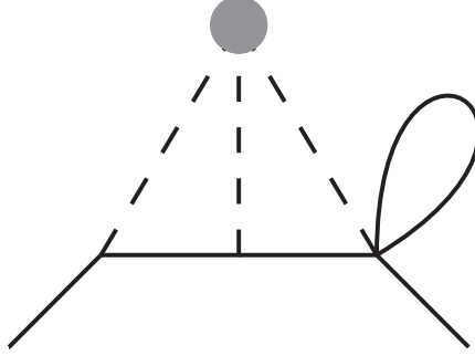
Figure 2: The graph corresponding to master integral J . Full (dashed) lines correspond to massive (massless) scalar propagators. The dot represents the influx of the external momentum q .
