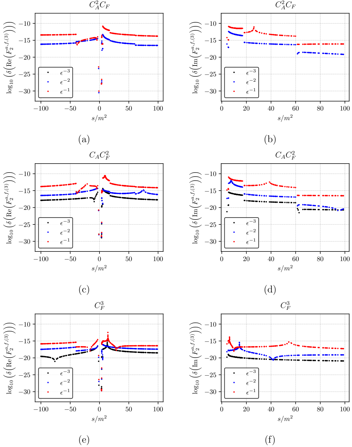
Figure 13: Relative cancellation of the real, (a), (c), (e), and imaginary parts, (b), (d), (f), of the poles for the non-fermionic colour structures of F_2^{a,f,(3)} , c.f. Eq. (31). Note that the 1/\epsilon^3 pole of the colour factor C_A^2 C_F is zero.
