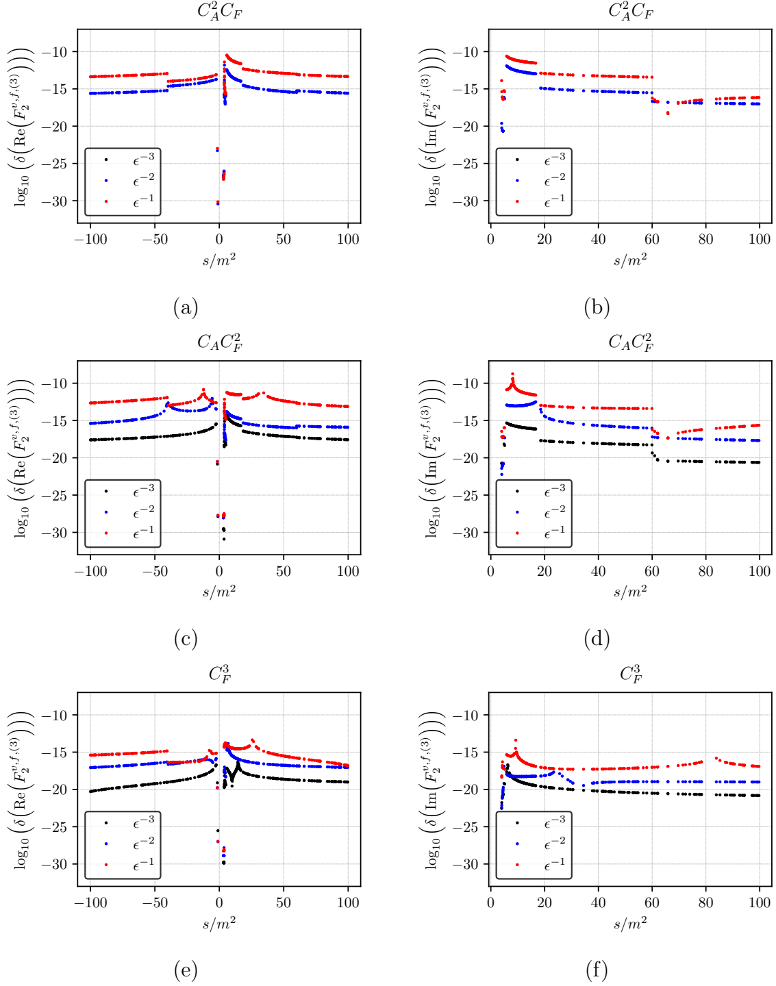
Figure 11: Relative cancellation of the real, (a), (c), (e), and imaginary parts, (b), (d), (f), of the poles for the non-fermionic colour structures of F_2^{v,f,(3)} , c.f. Eq. (31). Note that the 1/\epsilon^3 pole of the colour factor C_A^2 C_F is zero.
