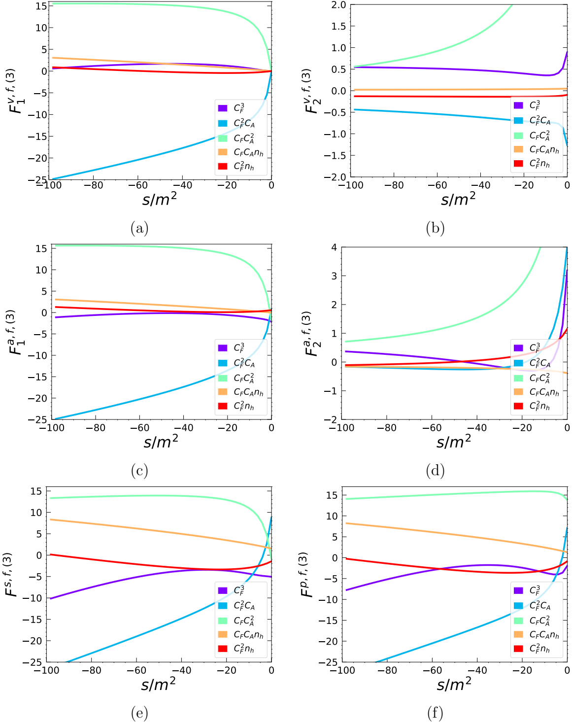
Figure 5: Non-singlet form factors as a function of s for s < 0 .
