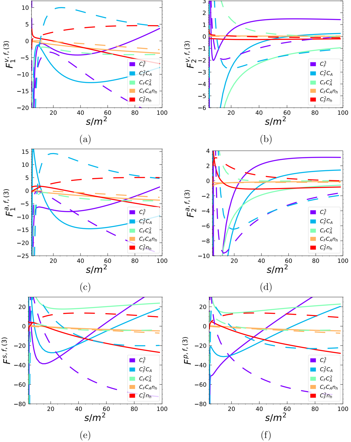
Figure 7: Non-singlet form factors as a function of s for s > 4m^2 . Real and imaginary parts are shown as solid and dashed lines, respectively.
