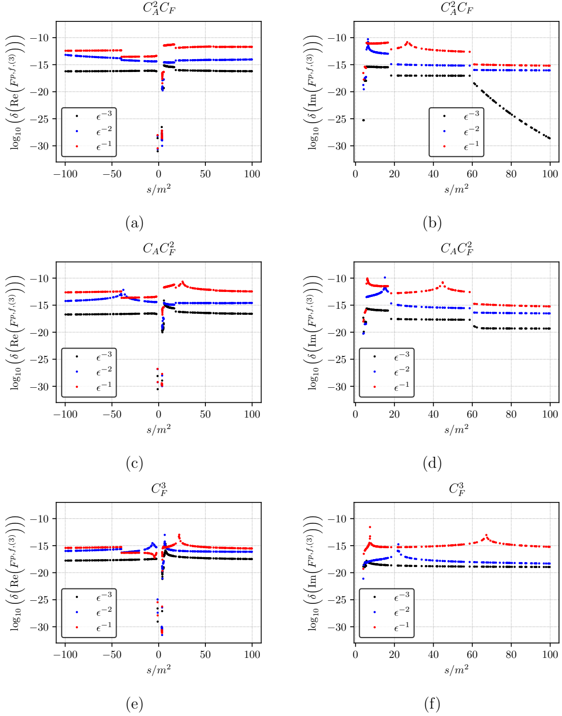
Figure 15: Relative cancellation of the real, (a), (c), (e), and imaginary parts, (b), (d), (f), of the poles for the non-fermionic colour structures of F^{p,f,(3)} , c.f. Eq. (31).
