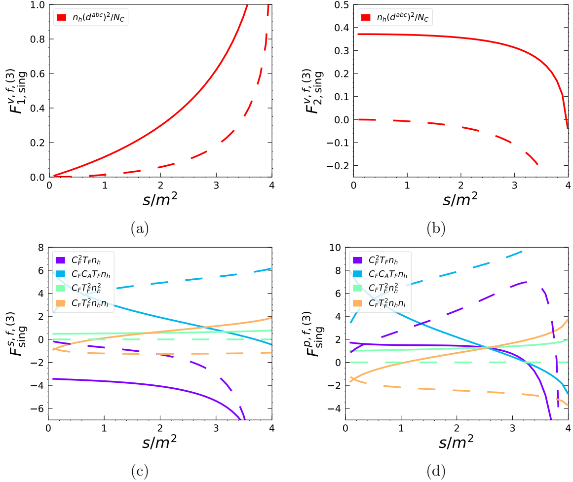
Figure 9: Singlet form factors as a function of s for 0 < s < 4m^2 . Real and imaginary parts are shown as solid and dashed lines, respectively.
