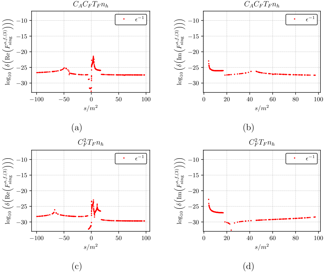
Figure 4: Relative cancellation of the real, (a), (c), and imaginary parts, (b), (d), of the poles for the colour structures C_A C_F T_F n_h and C_F^2 T_F n_h of F_{\text{sing}}^{s,f,(3)} , c.f. Eq. (31).
