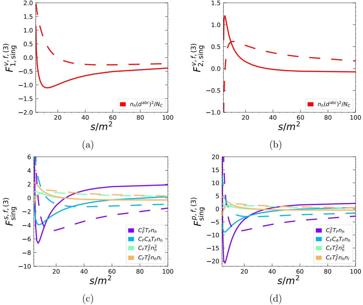
Figure 10: Singlet form factors as a function of s for s > 4m^2 . Real and imaginary parts are shown as solid and dashed lines, respectively.
