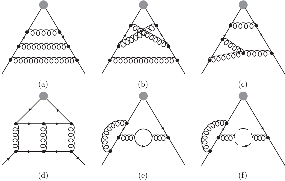
Figure 1: Sample diagrams contributing to the form factors. Solid, dashed and curly lines represent massive quarks, massless quarks and gluons, respectively. The blob refers to one of the external currents given in Eq. (1). Diagram (d) is a representative for the singlet contribution. Here the quark in the closed loop is massive.
