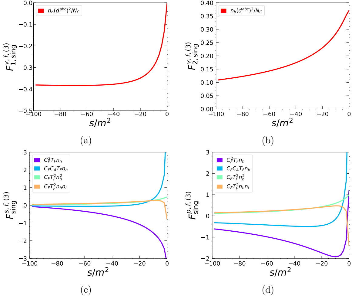
Figure 8: Singlet form factors as a function of s for s < 0 .
