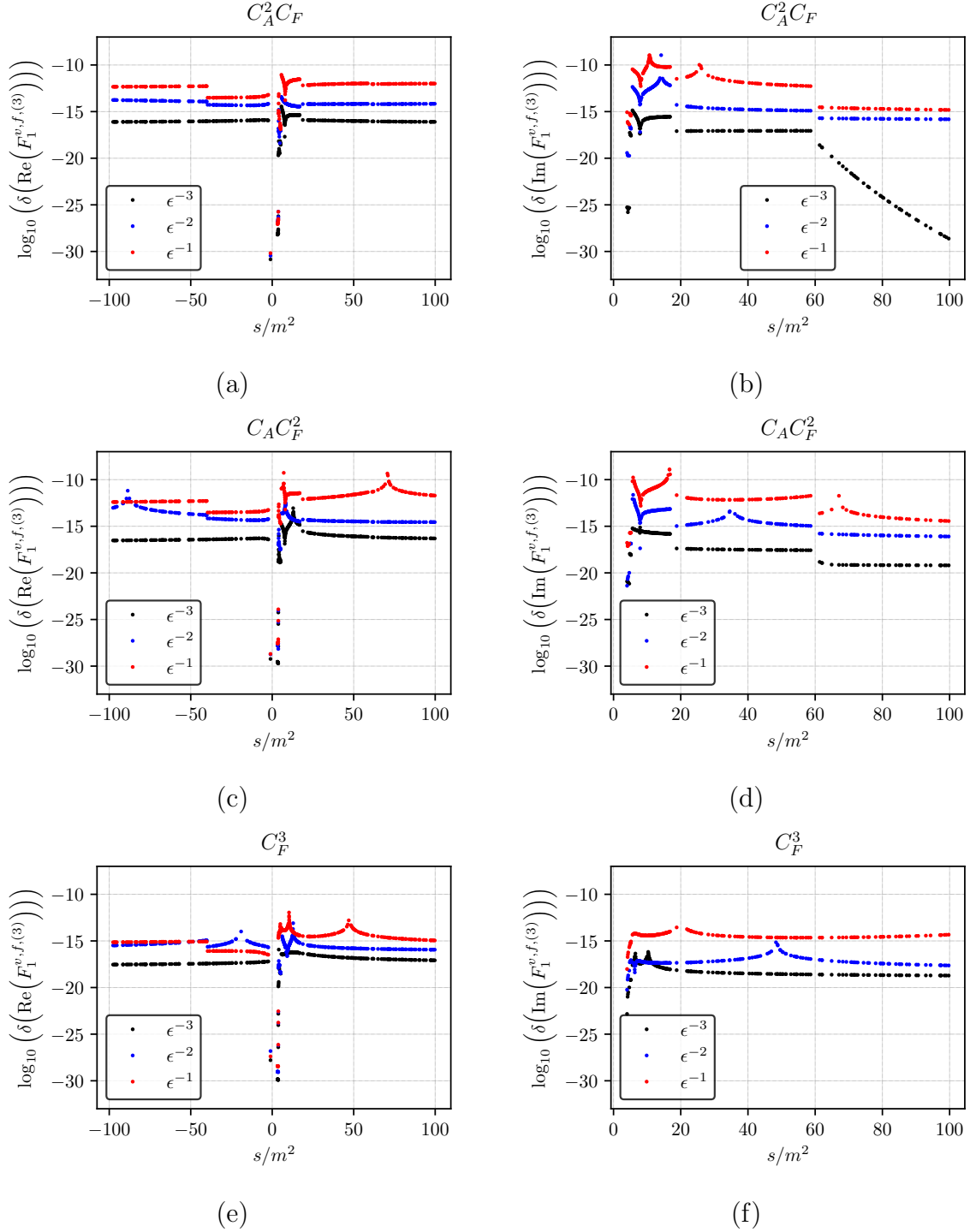
Figure 3: Relative cancellation of the real, (a), (c), (e), and imaginary parts, (b), (d), (f), of the poles for the non-fermionic colour structures of F_1^{v,f,(3)} , c.f. Eq. (31).
