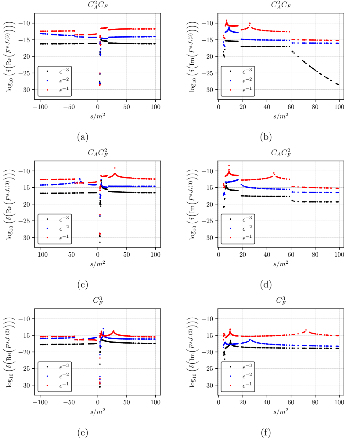
Figure 14: Relative cancellation of the real, (a), (c), (e), and imaginary parts, (b), (d), (f), of the poles for the non-fermionic colour structures of F^{s,f,(3)} , c.f. Eq. (31).
