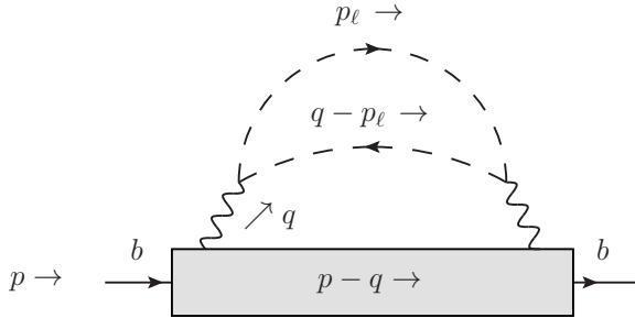
Figure 2: Our convention for the loop momentum routing. Charged lepton and neutrino momenta are p_\ell and q - p_\ell , respectively. The external bottom quark momentum is p . Additional loops of gluons and quarks are denoted generically with the gray blob. The arrows on the fermion lines indicate the fermion direction whereas the arrows next to the lines denote the momentum flow.
