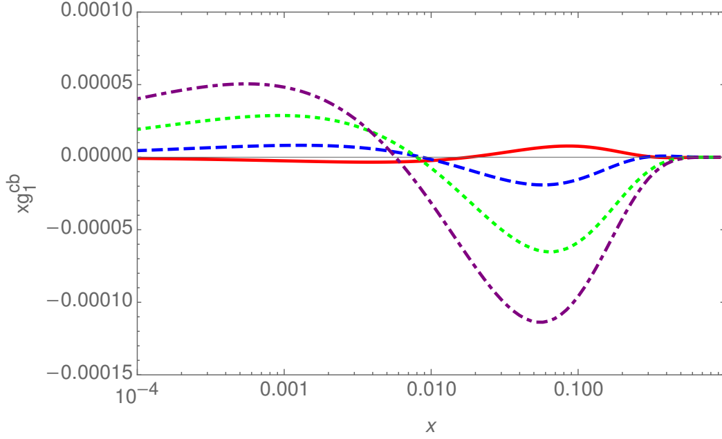
Figure 11: The O(a_s^2) two-mass contribution the polarized structure function xg_1(x, Q^2) as a function of x for Q^2 = 10 \text{ GeV}^2 (full line); 100 \text{ GeV}^2 (dashed line); 1000 \text{ GeV}^2 (dotted line), and 10000 \text{ GeV}^2 (dash-dotted line) for m_c = 1.59 \text{ GeV} and m_b = 4.78 \text{ GeV} and the parton distribution functions [27].
