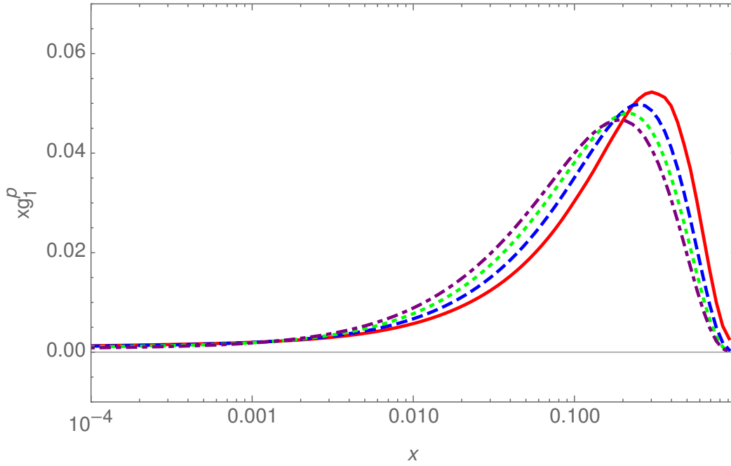
Figure 1: The NLO massless structure function xg_1(x, Q^2) as a function of x for Q^2 = 10 \text{ GeV}^2 (full line); 100 \text{ GeV}^2 (dashed line); 1000 \text{ GeV}^2 (dotted line), and 10000 \text{ GeV}^2 (dash-dotted line), using the parton distribution functions of [27].
