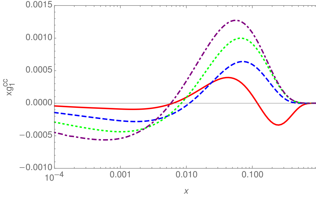
Figure 3: The O(a_s) charm contribution the polarized structure function xg_1(x, Q^2) as a function of x for Q^2 = 10 \text{ GeV}^2 (full line); 100 \text{ GeV}^2 (dashed line); 1000 \text{ GeV}^2 (dotted line), and 10000 \text{ GeV}^2 (dash-dotted line) for m_c = 1.59 \text{ GeV} and the parton distribution functions [27].
