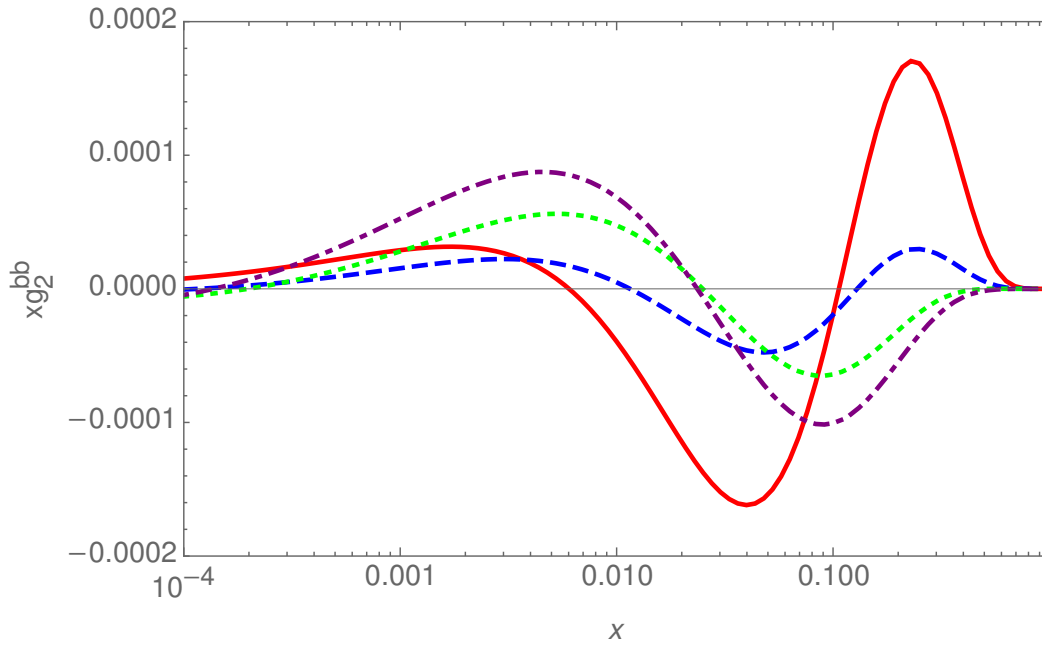
Figure 6: The O(a_s) bottom contribution the polarized structure function xg_2(x, Q^2) as a function of x for Q^2 = 10 GeV 2 (full line); 100 GeV 2 (dashed line); 1000 GeV 2 (dotted line), and 10000 GeV 2 (dash-dotted line) for m_b = 4.78 GeV and the parton distribution functions [27].
