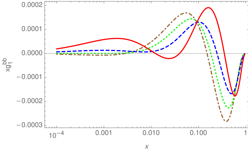
Figure 8: The O(a_s^2) bottom contributions to the structure function xg_1(x, Q^2) for m_b = 4.78 GeV as a function of x for Q^2 = 10 GeV 2 (full line); 100 GeV 2 (dashed line); 1000 GeV 2 (dotted line), and 10000 GeV 2 (dash-dotted line), using the parton distribution functions of [27].
