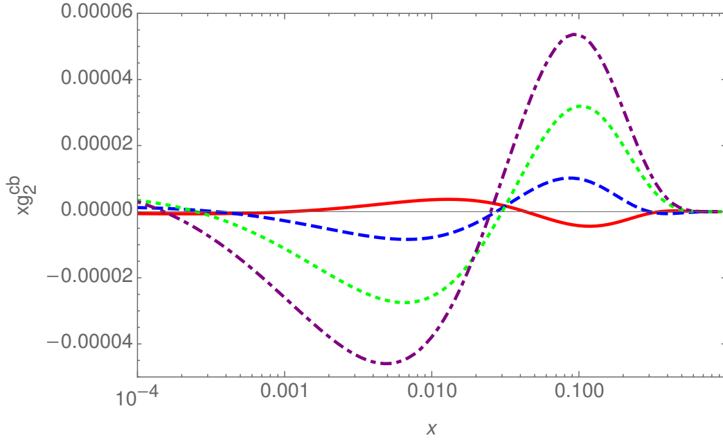
Figure 12: The O(a_s^2) two-mass contribution the polarized structure function xg_2(x, Q^2) as a function of x for Q^2 = 10 \text{ GeV}^2 (full line); 100 \text{ GeV}^2 (dashed line); 1000 \text{ GeV}^2 (dotted line), and 10000 \text{ GeV}^2 (dash-dotted line) for m_c = 1.59 \text{ GeV} and m_b = 4.78 \text{ GeV} and the parton distribution functions [27].
