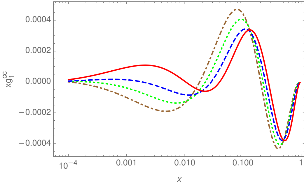
Figure 7: The O(a_s^2) charm contributions to the structure function xg_1(x, Q^2) for m_c = 1.59 GeV as a function of x for Q^2 = 10 GeV 2 (full line); 100 GeV 2 (dashed line); 1000 GeV 2 (dotted line), and 10000 GeV 2 (dash-dotted line), using the parton distribution functions of [27].
