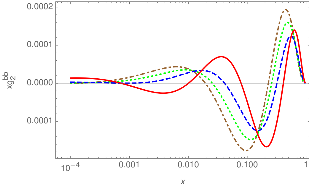
Figure 10: The O(a_s^2) bottom contributions to the structure function xg_2(x, Q^2) for m_b = 4.78 GeV as a function of x for Q^2 = 10 GeV 2 (full line); 100 GeV 2 (dashed line); 1000 GeV 2 (dotted line), and 10000 GeV 2 (dash-dotted line), using the parton distribution functions of [27].
