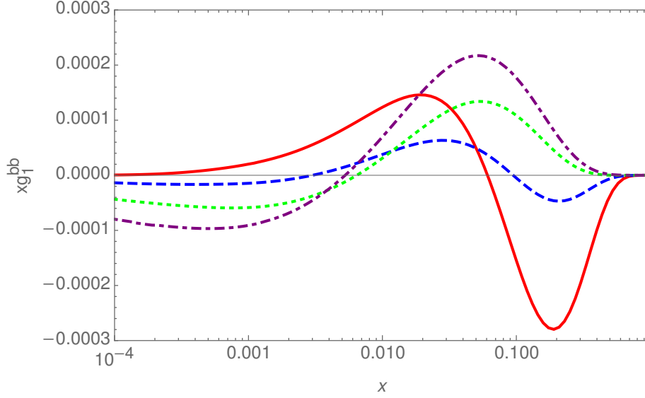
Figure 5: The O(a_s) bottom contribution the polarized structure function xg_1(x, Q^2) as a function of x for Q^2 = 10 GeV 2 (full line); 100 GeV 2 (dashed line); 1000 GeV 2 (dotted line), and 10000 GeV 2 (dash-dotted line) for m_b = 4.78 GeV and the parton distribution functions [27].
