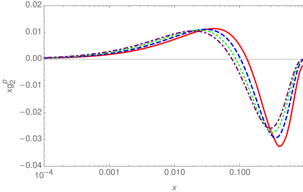
Figure 2: The NLO massless structure function xg_2(x, Q^2) as a function of x for Q^2 = 10 \text{ GeV}^2 (full line); 100 \text{ GeV}^2 (dashed line); 1000 \text{ GeV}^2 (dotted line), and 10000 \text{ GeV}^2 (dash-dotted line), using the parton distribution functions of [27].
