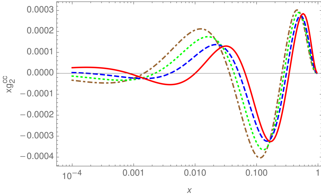
Figure 9: The O(a_s^2) charm contributions to the structure function xg_2(x, Q^2) for m_c = 1.59 GeV as a function of x for Q^2 = 10 GeV 2 (full line); 100 GeV 2 (dashed line); 1000 GeV 2 (dotted line), and 10000 GeV 2 (dash-dotted line), using the parton distribution functions of [27].
