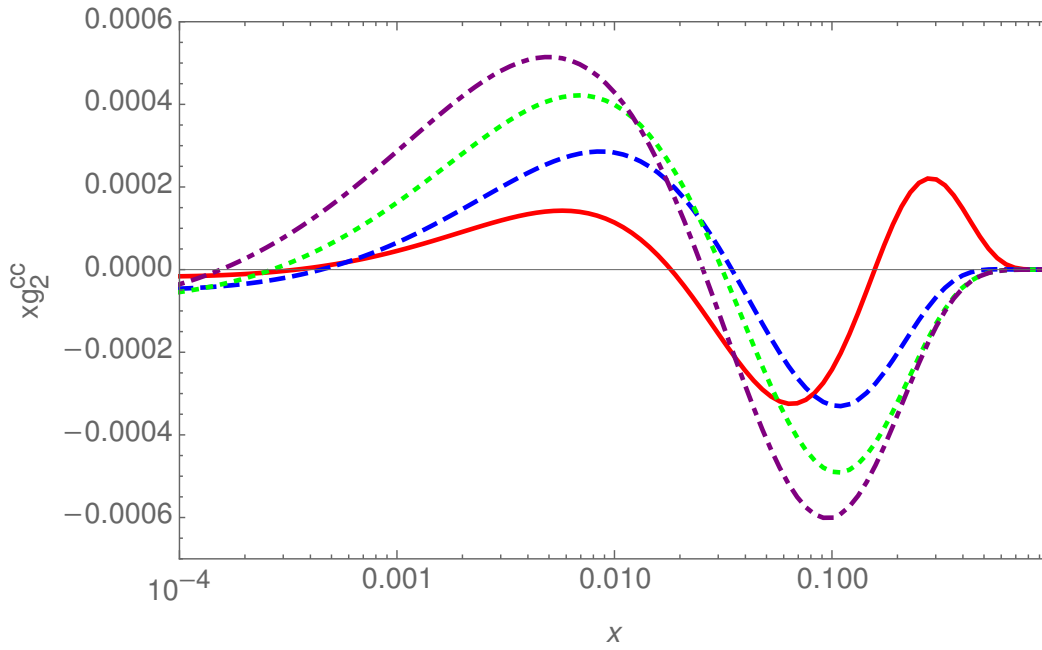
Figure 4: The O(a_s) charm contribution the polarized structure function xg_2(x, Q^2) as a function of x for Q^2 = 10 \text{ GeV}^2 (full line); 100 \text{ GeV}^2 (dashed line); 1000 \text{ GeV}^2 (dotted line), and 10000 \text{ GeV}^2 (dash-dotted line) for m_c = 1.59 \text{ GeV} and the parton distribution functions [27].
