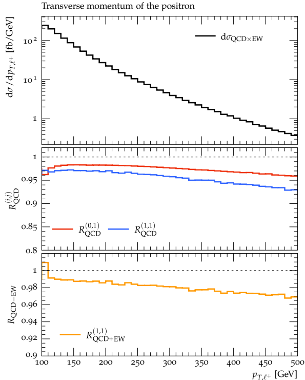
Figure 3. Transverse momentum distribution of the positively charged lepton. See the caption in Fig. 2 and the text for details.
