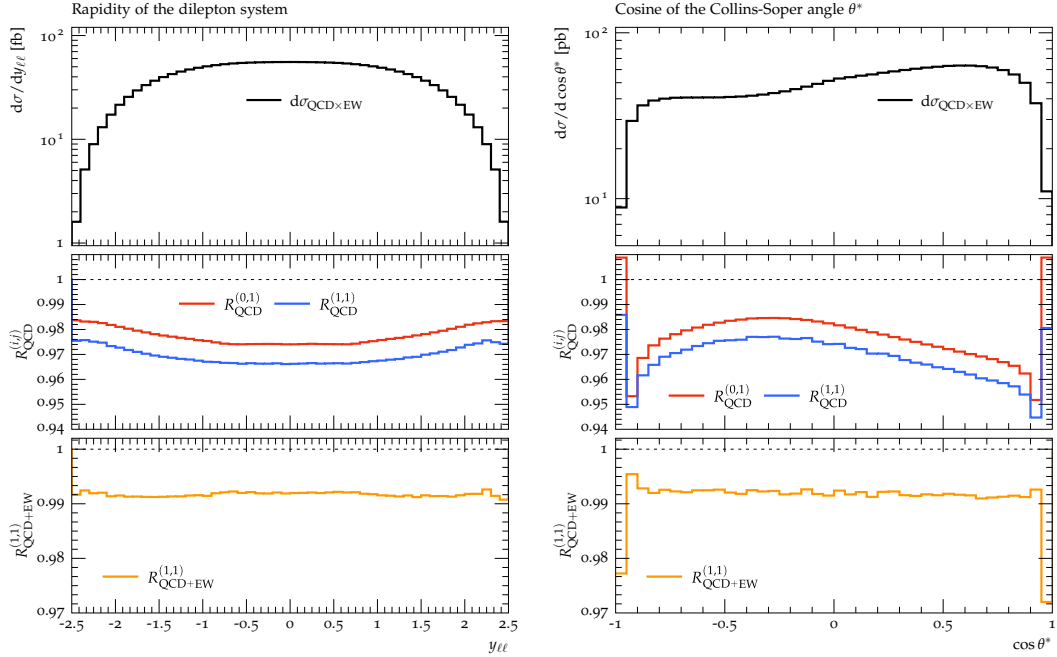
Figure 4. Distributions of the rapidity of the dilepton system and the cosine of the Collins-Soper angle. See the caption in Fig. 2 and the text for details.
