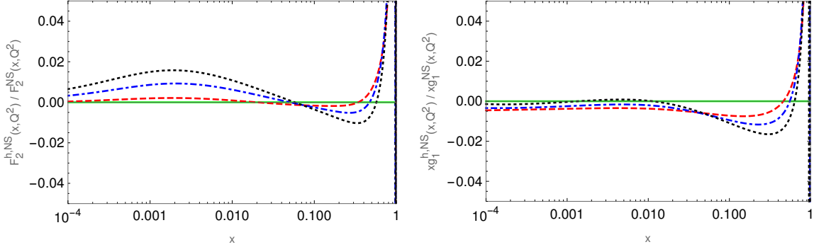
Figure 4: Left: The relative contribution of the heavy flavor contributions due to c and b quarks to the structure function F_2^{\text{NS}} at N^3\text{LO} ; dashed lines: 100 \text{ GeV}^2 ; dashed-dotted lines: 1000 \text{ GeV}^2 ; dotted lines: 10000 \text{ GeV}^2 . Right: The same for the structure function xg_1^{\text{NS}} at N^3\text{LO} . From [69].
