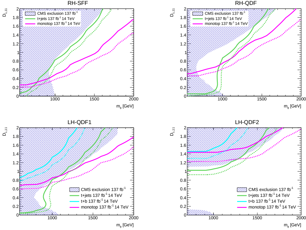
Figure 13: Full lines: excluded areas in the (m_\phi, D_{\lambda,11}) for the tj , tb and monoton analyses proposed in this paper for an integrated luminosity of 137 \text{ fb}^{-1} at a 14 TeV LHC. The excluded areas are on the left of the curves. The dashed lines show the corresponding results for 300 \text{ fb}^{-1} . The shaded area corresponds to the region excluded by the CMS analyses.
