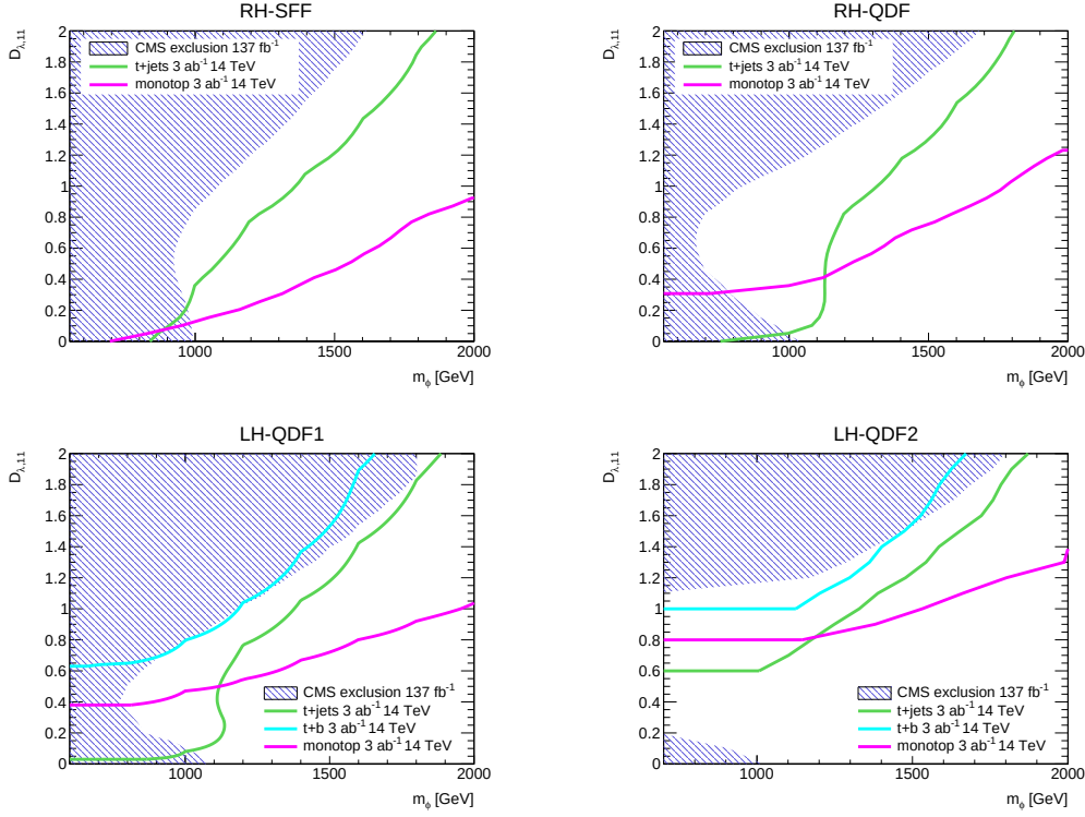
Figure 14: Excluded areas in the (m_\phi, D_{\lambda,11}) for the tj , tb and monotonop analyses proposed in this paper for an integrated luminosity of 3 \text{ ab}^{-1} at a 14 TeV LHC. The excluded areas are on the left of the curves. The shaded area corresponds to the region excluded by the CMS analyses.
