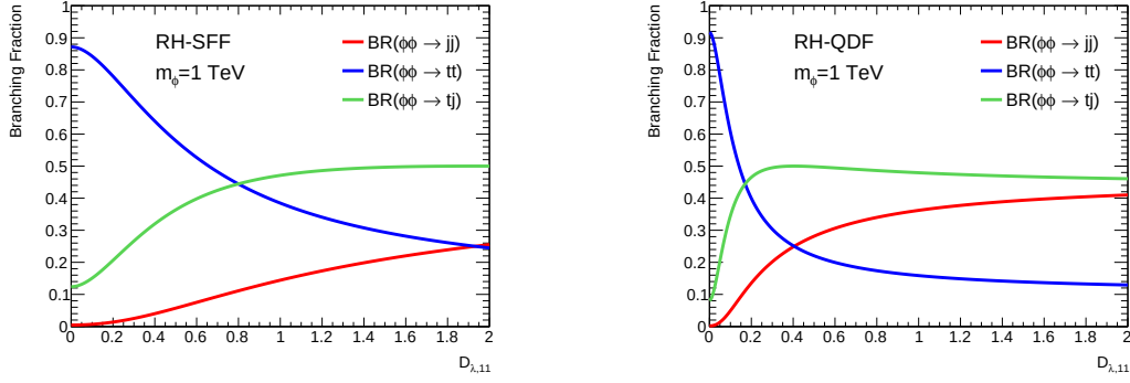
Figure 3: Branching fractions for three final states: jj + E_T^{\text{miss}} , t\bar{t} + E_T^{\text{miss}} and tj + E_T^{\text{miss}} as a function of the coupling D_{\lambda,11} for the two RH benchmarks. Left: RH-SFF benchmark; right: RH-QDF benchmark.
