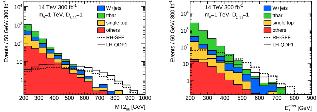
Figure 12: Distribution of the m_{T2} (left) and E_T^{miss} (right) variables for the tj and monotop analyses respectively for two signal points and for the SM backgrounds. The distributions are shown after all of the selection cuts are applied except the one on the plotted variable. The normalisation corresponds to an integrated luminosity of 300 \text{ fb}^{-1} .
