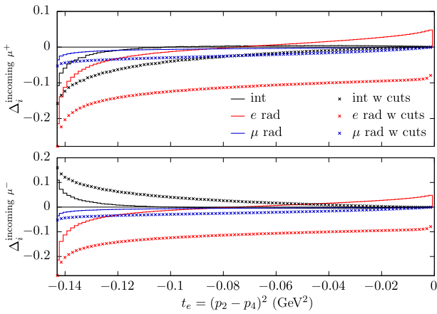
(a) d\sigma/dt_e
