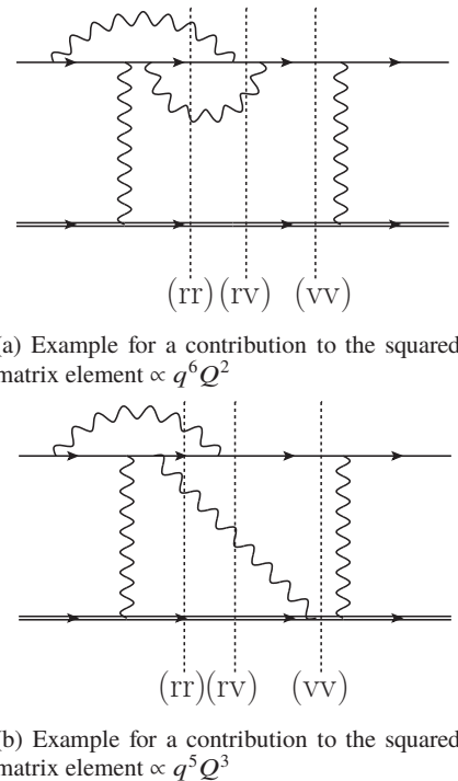
Fig. 5 Examples of NNLO QED contributions to \mathcal{M}_{n+2}^{(0)} (rr), \mathcal{M}_{n+1}^{(1)} (rv), and \mathcal{M}_n^{(2)} (vv). Analogous contributions with q^l Q^{8-l} with l \in \{4, 3, 2\} are understood.
