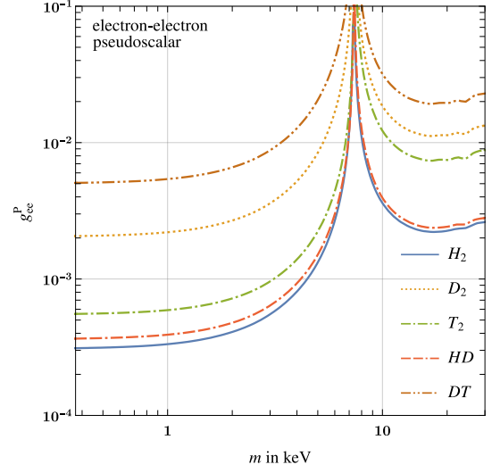
(b) Pseudoscalar electron–electron interaction.
