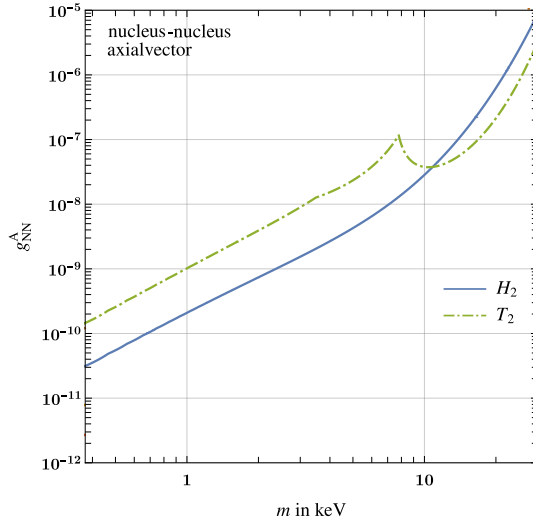
(c) Axialvector nucleus–nucleus interaction.
