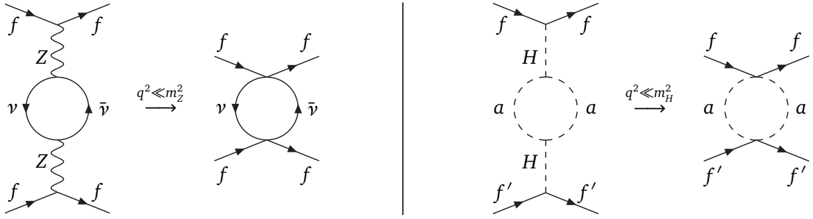
Figure 3: Longrange force mediated by double neutrino exchange (left) and double (Pseudo-)Goldstone boson exchange. In both cases, the direct coupling to the fermions is by a heavy particle ( Z or Higgs boson) leading to effective four-particle interactions.
