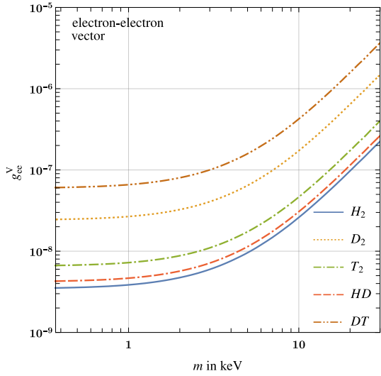
(a) Vector electron–electron interaction.
