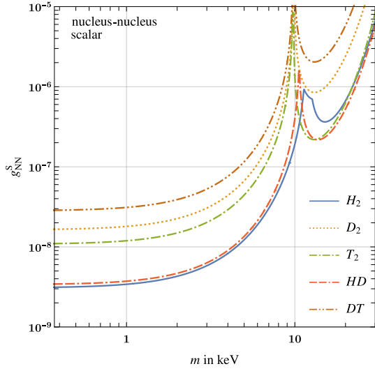
(c) Scalar nucleus–nucleus interaction.
