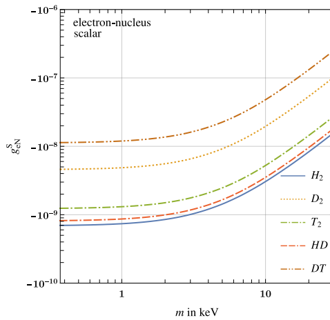
(e) Scalar electron–nucleus interaction with negative coupling g_{eN}^S < 0 .
