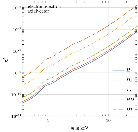
(b) Axialvector electron–electron interaction.
