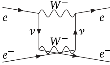
Figure 4: Additional contribution to the two-neutrino force induced by a W -box diagram.
