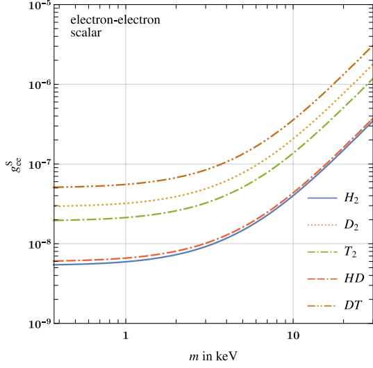
(a) Scalar electron–electron interaction.
