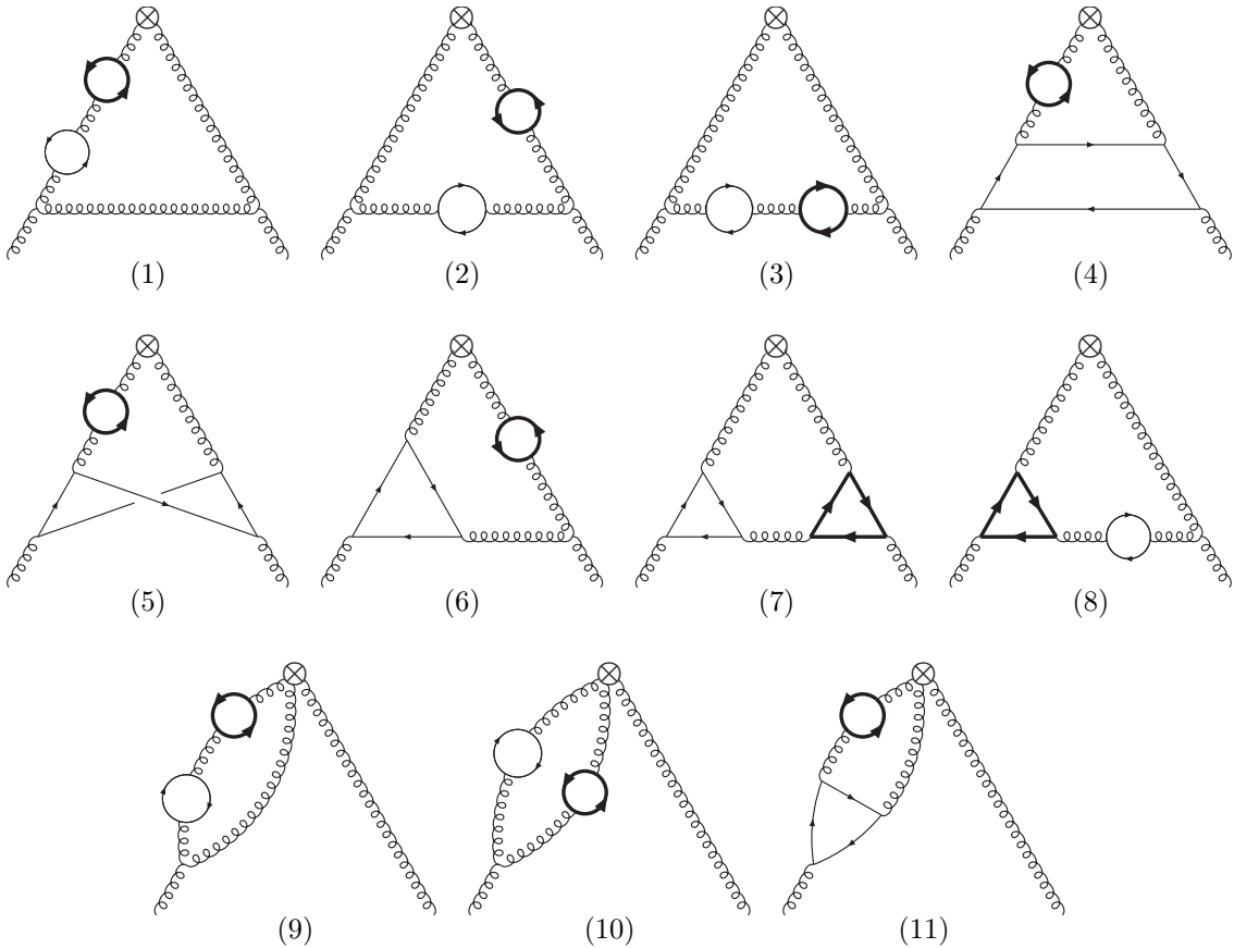
Figure 1: The 11 different topologies for \tilde{A}_{gg,Q}^{(3)} . Curly lines: gluons; thin arrow lines: lighter massive quark; thick arrow lines: heavier massive quark; the symbol \otimes represents the corresponding local operator insertion, cf. [55] for the related Feynman rules.
