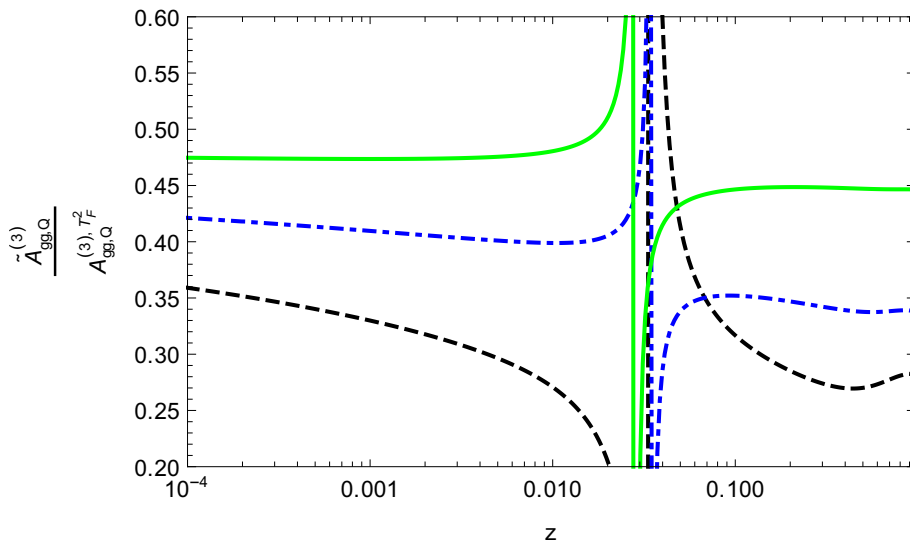
Figure 2: The ratio of the two mass contribution to the total contribution at O(T_F^2) for the polarized massive OME A_{gg,Q}^{(3)} as a function of the momentum fraction z and the virtuality \mu^2 . Dashed line: \mu^2 = 50 \text{ GeV}^2 ; Dash-dotted line: \mu^2 = 100 \text{ GeV}^2 ; Full line: \mu^2 = 1000 \text{ GeV}^2 . For the values of m_c and m_b we refer to the on-shell heavy quark masses m_c = 1.59 \text{ GeV} and m_b = 4.78 \text{ GeV} [71, 72].
