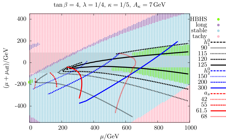
Figure 8: The behavior of the masses of the three lightest neutral Higgs states in a scenario with \lambda = 1/4 , \kappa = 1/5 , \tan\beta = 4 and A_\kappa = 7 \text{ GeV} is shown. In contrast to Figs. 4–7, the black and blue lines show the mass contours of the lightest and second lightest \mathcal{CP} -even Higgs mass eigenstate, respectively. The remaining parameters are chosen according to Tab. 1.
