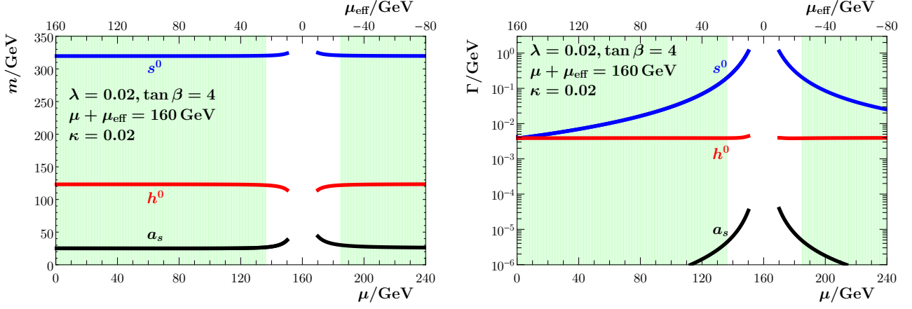
Figure 9: The mass spectrum (left) and total decay widths (right) for the three lightest Higgs bosons in a scenario with small \lambda = 0.02 and fixed \mu + \mu_{\text{eff}} = 160 GeV are shown. The value of \kappa is rescaled as \kappa \rightarrow \tilde{\kappa} according to Eq. (36) with \kappa = 0.02 . Furthermore, |A_\kappa| = 1.3 GeV with the opposite sign of \mu_{\text{eff}} . The other parameters are given in Tab. 1. The green area indicates compatibility with the constraints from HiggsSignals.
