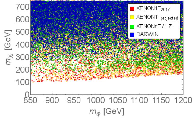
Figure 7.2: Viable area in the m_\phi - m_{\chi_t} plane of the quark doublet DMFV model with combined flavour, relic abundance and direct detection constraints applied in the QDF scenario, for \eta = -0.01 . We show the viable ranges for different strengths of direct detection bounds. The current exclusion bounds of XENON1T [36] as well as the projected bounds of XENON1T [38], XENONnT [38], LUX-ZEPLIN (LZ) [39] and DARWIN [40] are applied respectively. The interference of relic abundance and direct detection effects results in a lower bound on the DM mass, increasing with more stringent direct detection bounds.
