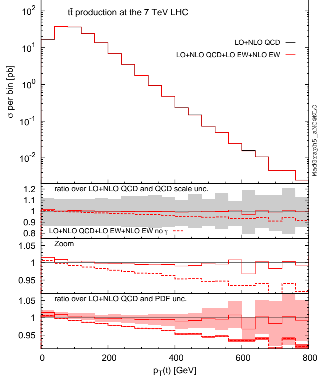
Figure 3: Comparison of QED and weak corrections, prepared by Davide Pagani and Marco Zaro using MadGraph5_aMC@NLO [?].
