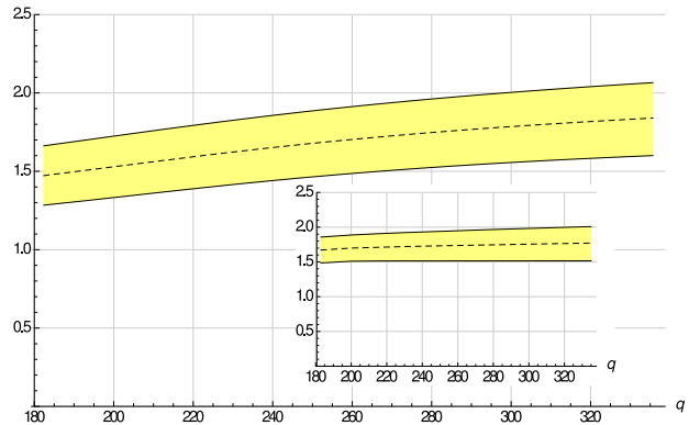
Figure 2: Main plot: NLO K -factor for gg \rightarrow ZZ production through the top quark loop as a function of the invariant mass of the Z -boson pair q , in GeV. Inset: NLO K -factor for gg \rightarrow H as a function of the Higgs boson mass q , in GeV. Bands correspond to variations of the renormalization and factorization scales in the interval q/4 \leq \mu \leq q . The dashed line shows the K -factors computed for the renormalization and factorization scales set to \mu = q/2 . We used the program MCFM [27] to compute the K -factor for the Higgs boson production.
