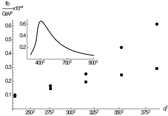
Figure 3: LO pp \rightarrow ZZ production cross-section (gluon fusion through top loop only) d\sigma/dq^2 in \text{fb}/\text{GeV}^2 , as a function of the invariant mass squared of the Z -boson pair, q^2 , in \text{GeV}^2 with a top mass of 173 GeV. We compare our cross-section, which is valid in the m_t \rightarrow \infty limit, with the one implemented in MCFM, which has exact m_t dependence. The dots and squares correspond to the results from MCFM and this paper respectively. We set the renormalization scale and the factorization scale to 200 GeV. The difference between the values ranges from \sim 20\% to \sim 220\% for the values of q^2 considered. The inset shows the MCFM cross-section computed for a larger range of the invariant masses.
