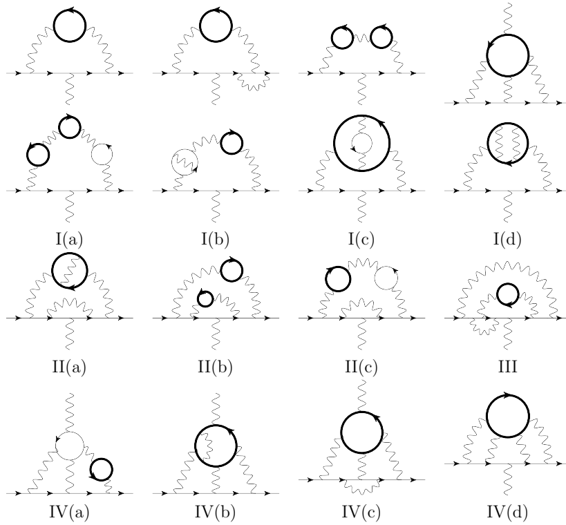
Figure 4: Sample Feynman diagrams contributing to a_\mu . Thin and thick solid lines represent light and heavy leptons, respectively.
