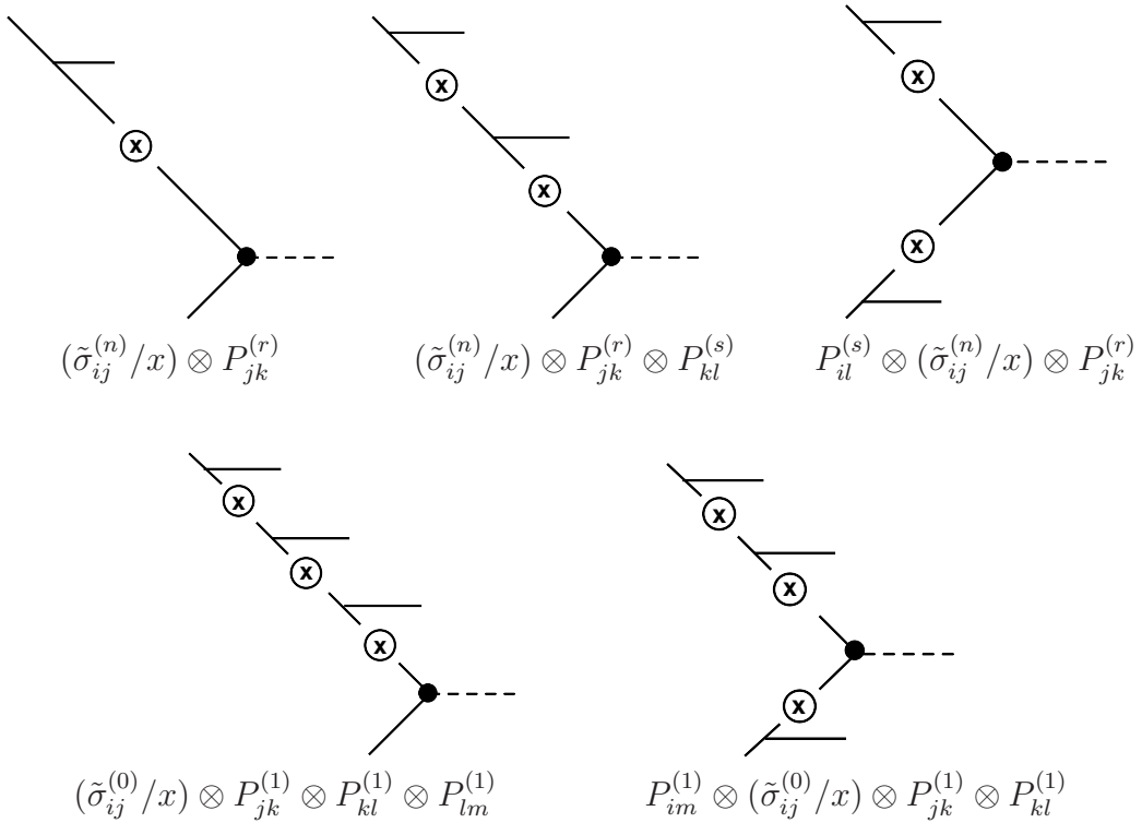
Figure 1: Schematic representation of the convolutions of the partonic cross section \tilde{\sigma}_{ij} with the splitting functions P_{jk} .
