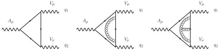
Figure 1: Sample diagrams that contribute to \langle VVA \rangle correlator at one, two and three-loops. The momenta q_{1,2} are outgoing.
