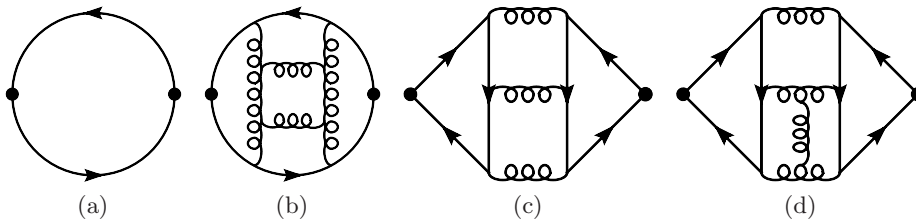
Figure 1: Examples of a lowest order and five-loop non-singlet (a),(b) and singlet (c),(d) diagrams contributing to the vector correlator.
