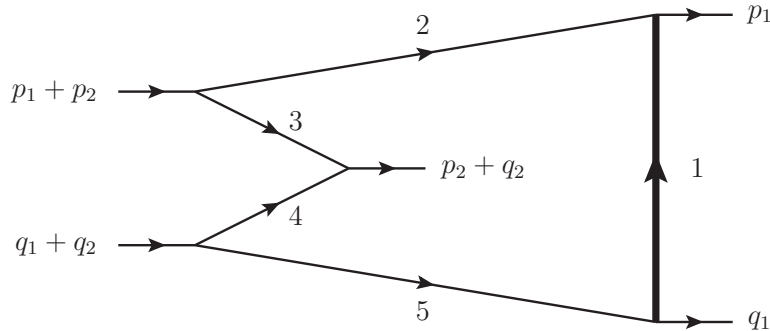
Figure 1: One-loop five-point integral exhibiting a Glauber contribution.
