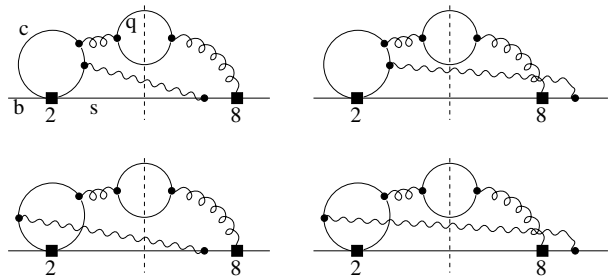
FIG. 1: Feynman diagrams that determine K_{28}^{(2)\beta_0} .
