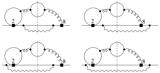
FIG. 2: Feynman diagrams excluded from K_{28}^{(2)\beta_0} .
