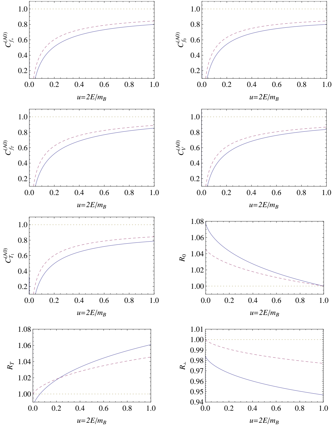
Figure 3: The A0 -type coefficients C_X^{(A0)} and the ratios R_X ( X = 0, T, \perp ) defined in (58) as a function of u (related to light-meson energy E = um_B/2 or momentum transfer q^2 = (1-u)m_B^2 ), with the scales fixed at \nu = \mu = m_b . The legend is the same as in Figure 2.
