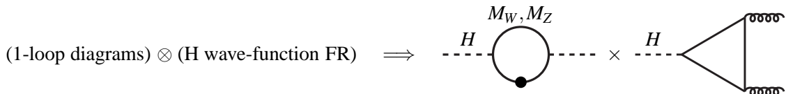
Figure 1: Singular \beta^{-1} behavior at the normal m threshold coming from WFR.
