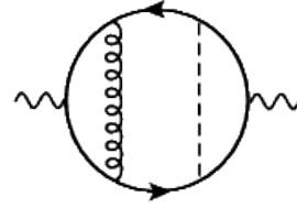
Figure 1: Sample diagram for the \alpha_s X_t^2 f(M_t/M_H) contribution. Solid lines denote top quarks, dashed lines Higgs or Goldstone bosons and curly lines gluons.
