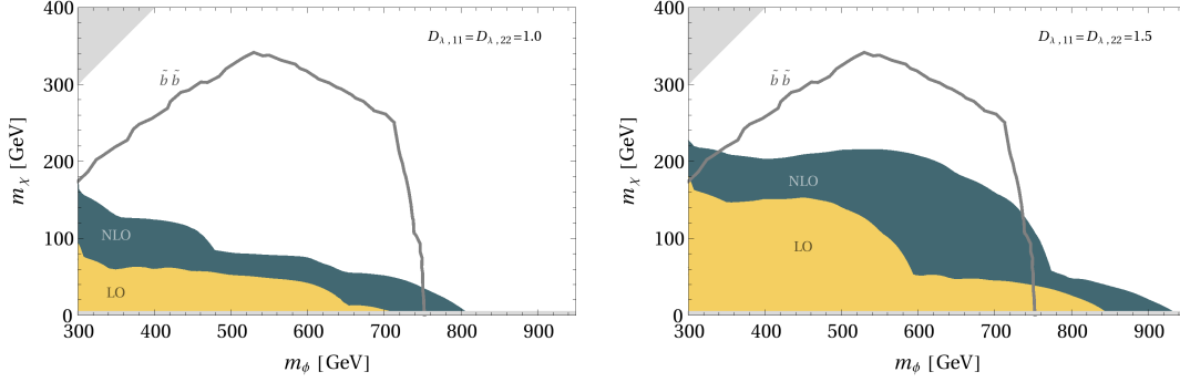
Figure 6: Limits on DMFV from the CMS 19.5 \text{ fb}^{-1} sbottom [10] and squark [11] search. The DM coupling to b -quark, D_{\lambda,33} is fixed everywhere by the corresponding relic abundance constraint, and all mixing angles are set to zero for simplicity.
