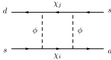
Figure 2: New contribution to K^0 - \bar{K}^0 mixing in DMFV.
