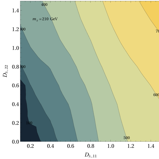
Figure 7: Limits on DMFV in terms of mass of \phi (in GeV) from the CMS monojet search [13].
