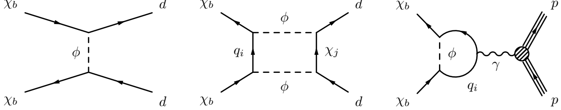
Figure 4: Diagrams contributing to WIMP-nucleon scattering in the mDMFV model.
