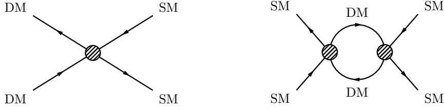
Figure 1: Schematic diagrams contributing to experimental constraints on flavoured DM.
