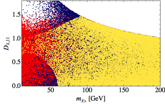
Figure 5: First generation coupling D_{\lambda,11} as functions of the DM mass m_{\chi_b} . The red points satisfy the bound from LUX, while the blue points satisfy the flavour constraints. For the yellow points both LUX and flavour constraints are imposed.
