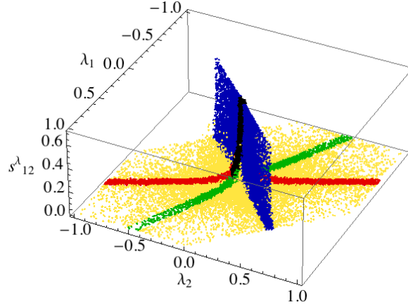
Figure 3: Allowed ranges for the mixing angle s_{12}^\lambda = \sin \theta_{12}^\lambda as a function of the non-universality parameters \lambda_1 and \lambda_2 . The five scenarios are: universality (black), small mixing (yellow), 12-degeneracy (blue), 13-degeneracy (red), 23-degeneracy (green).
