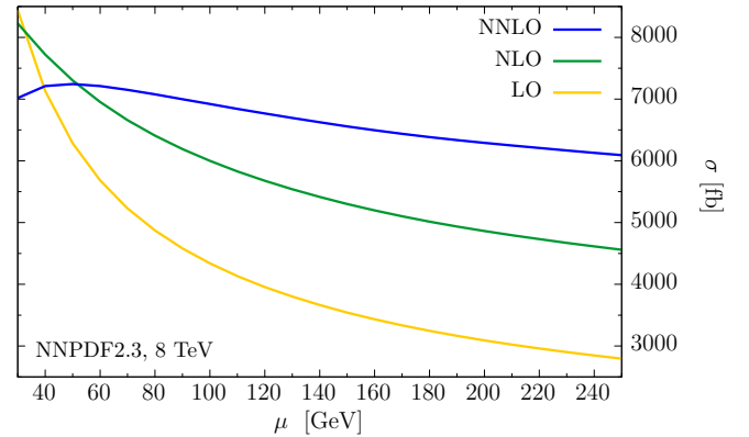
Figure 2: Dependence of the total LO, LO and NNLO cross-sections on the unphysical scale \mu . See text for details.
