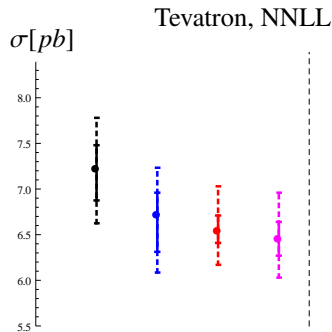
Figure 11: Top-pair production cross section calculations with NNLL accuracy in p\bar{p} collisions at \sqrt{s} = 1.96 TeV (Tevatron). To the left of the dashed line: NNLO app + NNLL results. Black: Beneke et al. [117] and TOPICS 1.0 ( m_t = 173.3 GeV); Blue: Cacciari et al. [127] ( m_t = 173.3 GeV) Red: Ahrens et al. [129] (1PI, m_t = 173.1 GeV) Magenta: Ahrens et al. [129] (PIM, m_t = 173.1 GeV) To the right of the dashed line: full NNLO + NNLL results. Black: Update of Beneke et al. [133] and TOPICS 2.0 ( m_t = 173.3 GeV) Blue: Czakon et al. [132] and top++2.0 ( m_t = 173.3 GeV) Darkgreen: CDF/D0 combined measurement quoted from CMS/ATLAS-CONF-2012-149. Error bars: inner solid – theory uncertainty of the partonic cross section excluding \alpha_s , outer dashed – PDF ( +\alpha_s ) added. PDF set: MSTW2008 NNLO with \alpha_s(M_Z) = 0.1171 \pm 0.0014 .
