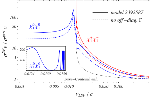
Figure 17: The enhancement of the \chi_1^0\chi_1^0 and \chi_1^+\chi_1^- annihilation cross sections for Snowmass model 2392587 relative to the perturbative tree-level rate, (\sigma^{\text{SF}}_{\nu})/(\sigma^{\text{pert}}_{\nu}) . The solid lines refer to the calculation of the Sommerfeld-enhanced rates with off-diagonal entries in the annihilation matrices included. The dashed curves show the enhancement with respect to the perturbative cross sections when off-diagonal annihilation rates are not considered. The dotted curve labelled “pure-Coulomb enh.” shows the enhancement from photon exchange only in the \chi_1^+\chi_1^- channel. Figure from [168].
