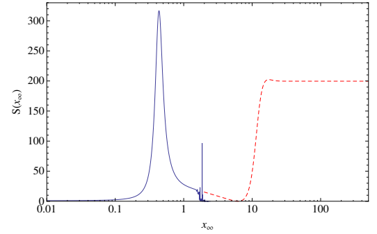
Figure 16: S-wave spin-0 Sommerfeld factor for v = 0.012 in a wino-like model as described in the text. The light-grey (red) dashed curve shows S(x_\infty) , when only the \chi_1^0 \chi_1^0 and \chi_1^+ \chi_1^- two-particle states in the Schrödinger equation and the annihilation process are kept and the asymptotic regime is reached for x_\infty > 50 . The dark-grey (blue) solid curve shows the result when the \chi_1^0 \chi_2^0 state is included. In this case, the evaluation fails for x_\infty > 2 and no reliable result is obtained. Figure from [167].
