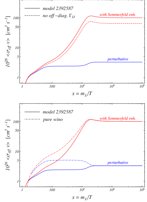
Figure 18: Upper panel: The thermally averaged effective annihilation rate \langle\sigma_{\text{eff}}\nu\rangle as a function of the scaled inverse temperature x = m_{\chi}/T for Snowmass model 2392587. The two upper (red) curves correspond to the Sommerfeld-enhanced annihilation cross sections including (solid line) or neglecting (dashed line) the off-diagonals in the annihilation matrices. The lower (blue) curve represents \langle\sigma_{\text{eff}}\nu\rangle obtained from perturbative (tree-level) cross sections. Lower panel: Comparison of \langle\sigma_{\text{eff}}\nu\rangle for model 2392587 (solid) with the corresponding pure-wino scenario (dot-dashed). Figures from [168].
