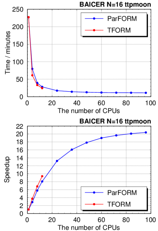
Figure 13: Comparison of timing and speedup for ParFORM and TFORM running on ttpmoon .
