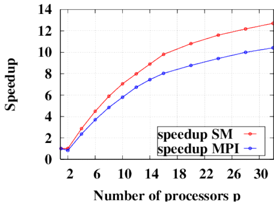
Figure 8: Runtime and speedup for the test program BAICER running on a SGI Altix 3700 server with 32 Itanium-2 processors (1.3 GHz). The lower curve corresponds to the MPI version and the upper one to the shared memory version of ParFORM.
