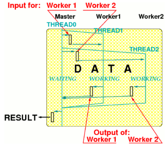
Figure 11: Mode of operation for TFORM.
