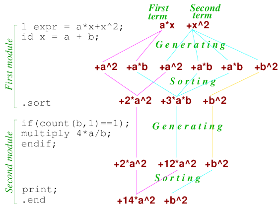
Figure 4: Example for the generation and sorting of data in FORM.
