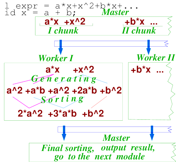
Figure 5: General conception of ParFORM.
