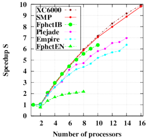
Figure 10: The speedup for the test program on different clusters in comparison to the SMP computer (cf. Fig. 8).
