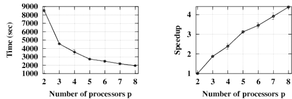
Figure 1: Speedup for the program BAICER on Compaq-AlphaServer with 8 Alpha (EV67) processors with 700 MHz.
