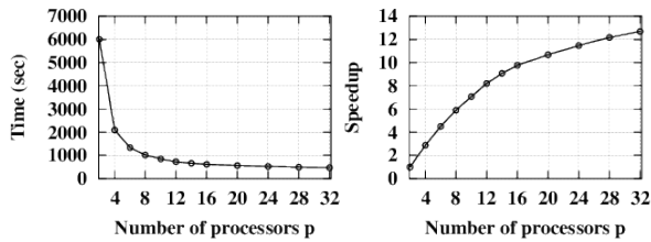
Figure 2: Computing time and speedup for the test program BAICER on the SGI Altix 3700 server with 32x Itanium-2 processors (1.3 GHz).
