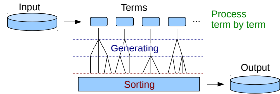
Figure 3: Graphical representation of the processing of an input expression in FORM.
