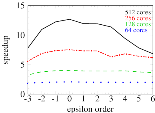
Figure 16: Speedup of the calculation of the various \epsilon orders of Feynman diagram given in Fig. 15 using 64 (dotted), 128 (dashed), 256 (dash-dotted) and 512 (solid) cores normalized to the 32-core run.
