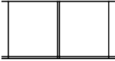
Figure 14: Integral family with three massive (double lines), three massless lines and an irreducible numerator (not shown). It is evaluated in forward-scattering kinematics, i.e., there is one external momentum, p_1 , flowing through the upper massless line and another, p_2 , through the lower massive lines.
