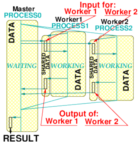
Figure 7: Mode of operation implemented into ParFORM for a NUMA architecture.
