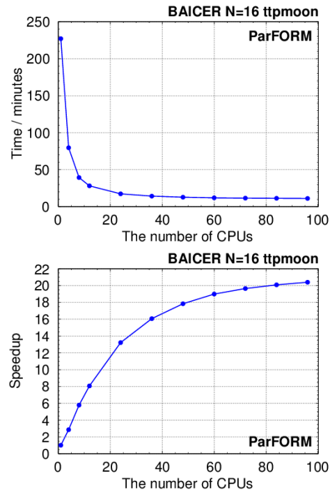
Figure 9: Timing and speedup plot for the ParFORM benchmark job BAICER running on ttpmoon .
