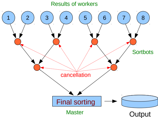
Figure 12: Illustration of the mode of operation of sortbots.
