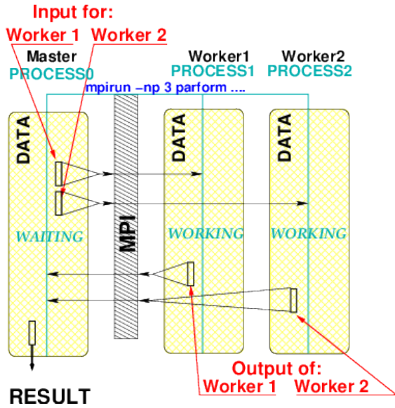
Figure 6: Visualization of the mode of operation of ParFORM based on MPI.
