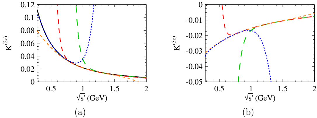
Figure 3: (a) Comparison of exact result (solid, black) for K^{(2c)}(s, s') and the various approximations for s \gg s' (blue, dotted), s \approx s' (orange and red, short and medium dashed) and s \ll s' (green long dashed) for \sqrt{s} = 1 GeV as a function of \sqrt{s'} . (b) Approximations for K^{(3c)}(s, s') .
