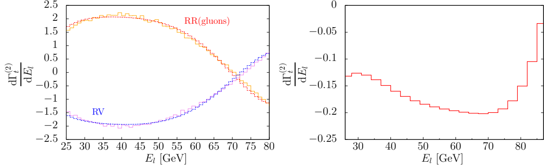
Figure 1. Distribution of the second order coefficient d\Gamma_t^{(2)} in the positron energy. Left pane: double-real and real-virtual contributions. Original histograms are shown with solid lines; Legendre polynomial fit is shown with dashed lines. Right pane: distribution of d\Gamma_t^{(2)} in the lepton energy. See text for details.
