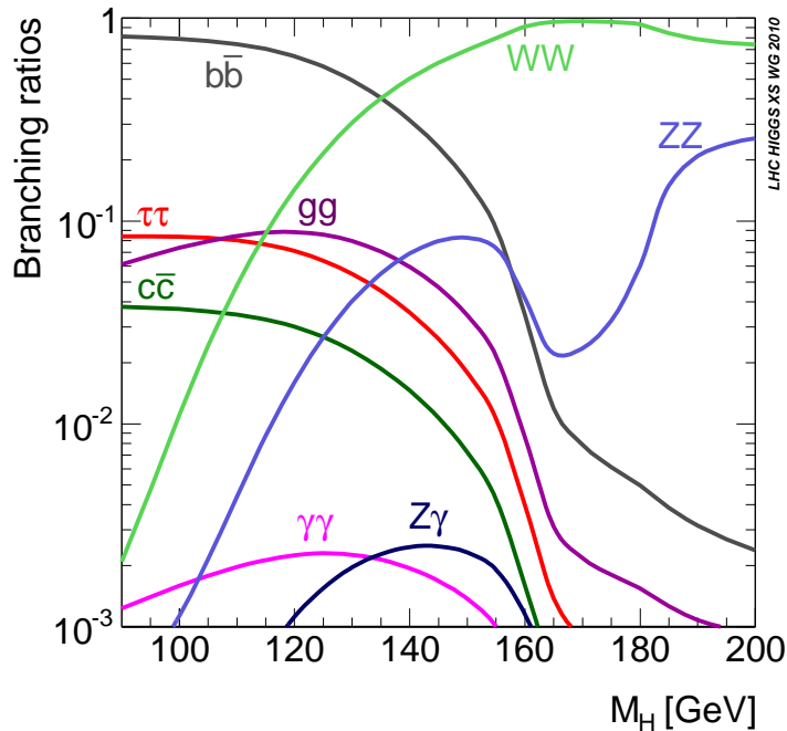
Figure 8.1: Higgs boson branching ratios in the SM at the LO from Ref. [273].
