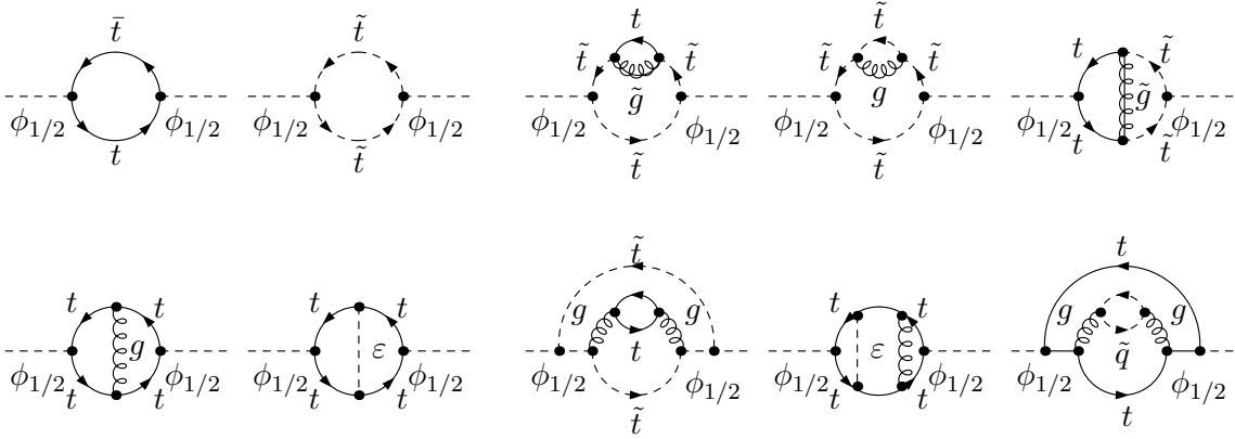
Figure 7.4: Sample diagrams contributing to \Sigma_{\phi_1}, \Sigma_{\phi_2}, \Sigma_{\phi_1\phi_2} , etc. to one-, two- and three-loops. Internal solid, dashed, dotted and curly lines correspond to top quarks, top squarks, \varepsilon -scalar and gluons, respectively. Gluinos are depicted with as curly lines with an additional solid line in the middle. The external dashed line corresponds to the Higgs bosons.
