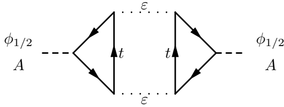
Figure 7.5: Sample diagram contributing a finite term to \Sigma_{\phi_1} , \Sigma_{\phi_2} , etc. when the infra-red divergence are regulated through a small external momentum or a finite \varepsilon -scalar mass.
