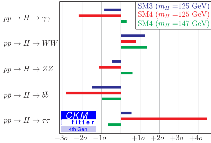
Pulls of the Higgs signal strengths
