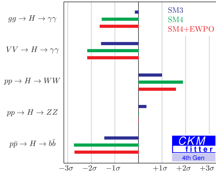
Pulls of the Higgs signal strengths
