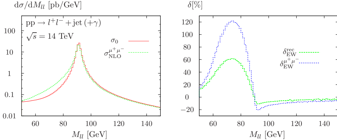
Figure 1: EW corrections (right) to the invariant-mass distribution of the lepton pair (left). Corrections for bare muons ( \delta_{\text{EW}}^{\mu^+\mu^-} ) and for recombination of collinear lepton–photon pairs ( \delta_{\text{EW}}^{\text{rec}} ) are shown.
